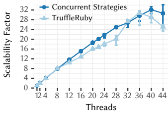
Fig. 12. Scalability of the parallel Mandelbrot benchmark, relative to 1-thread performance of TruffleRuby.
