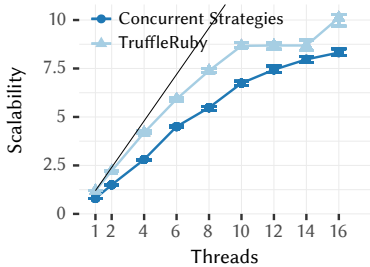
Fig. 15. Scalability of the Sidekiq PDF Invoice benchmark with Concurrent Strategies, relative to 1-thread performance of TruffleRuby.
