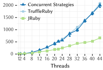
Fig. 13. Scalability of the threaded reverse benchmark, relative to 1-thread performance of each implementation.
